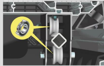
Strong and steady working table with double handle: • Its slides on 2 steel square rails with 6 wheels; 4 up and 2 down; • Every wheels has 2 ball bearings for a total of 12.
